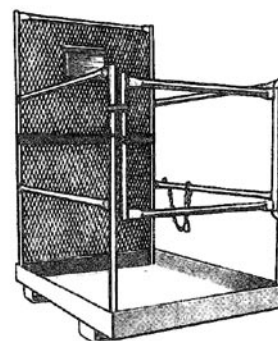
Forklift work platform has standard guardrails and a screen to prevent contact with moving parts of the mast. A chain secures the platform to the mast.
